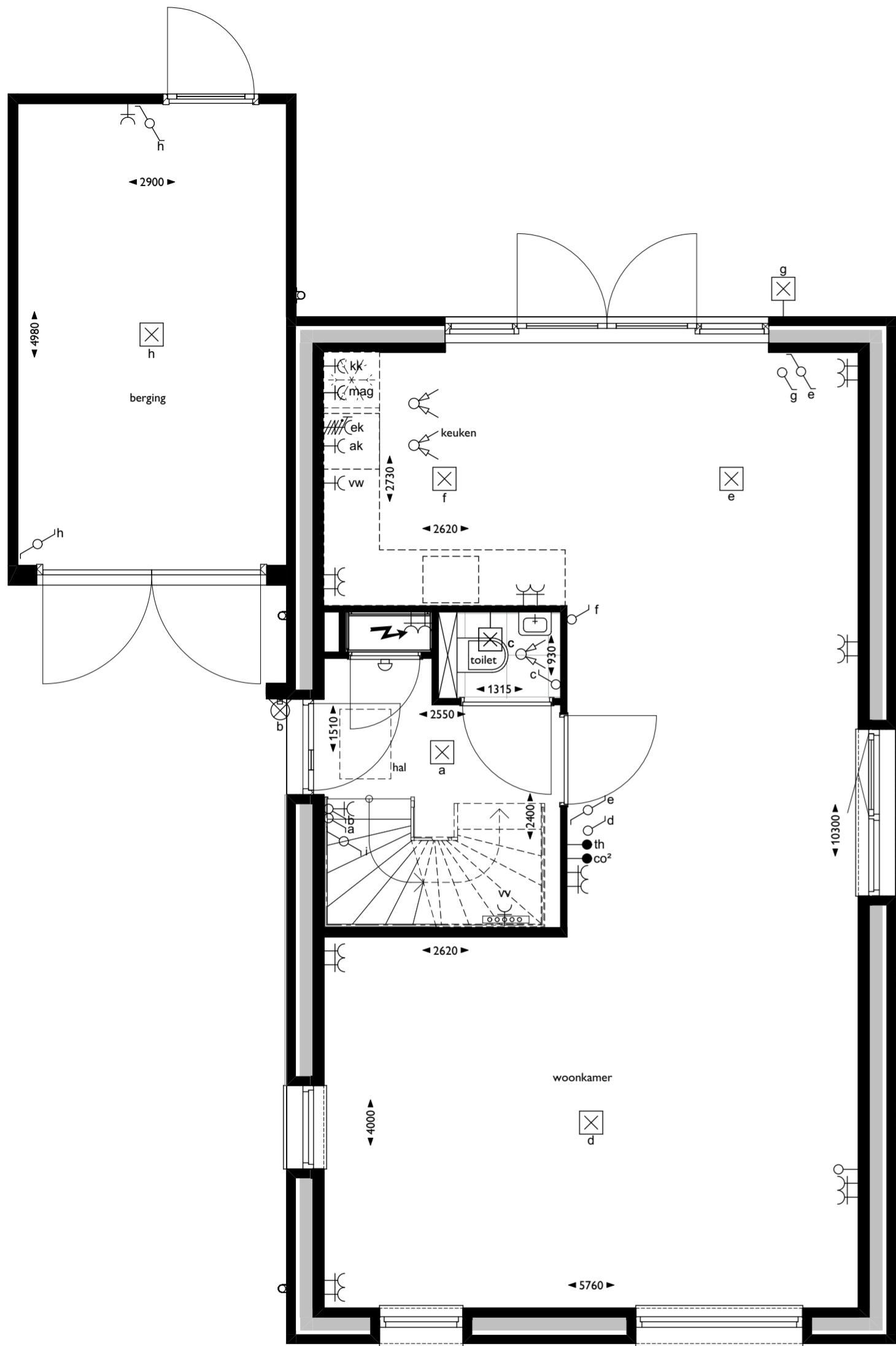
00 begane grond
