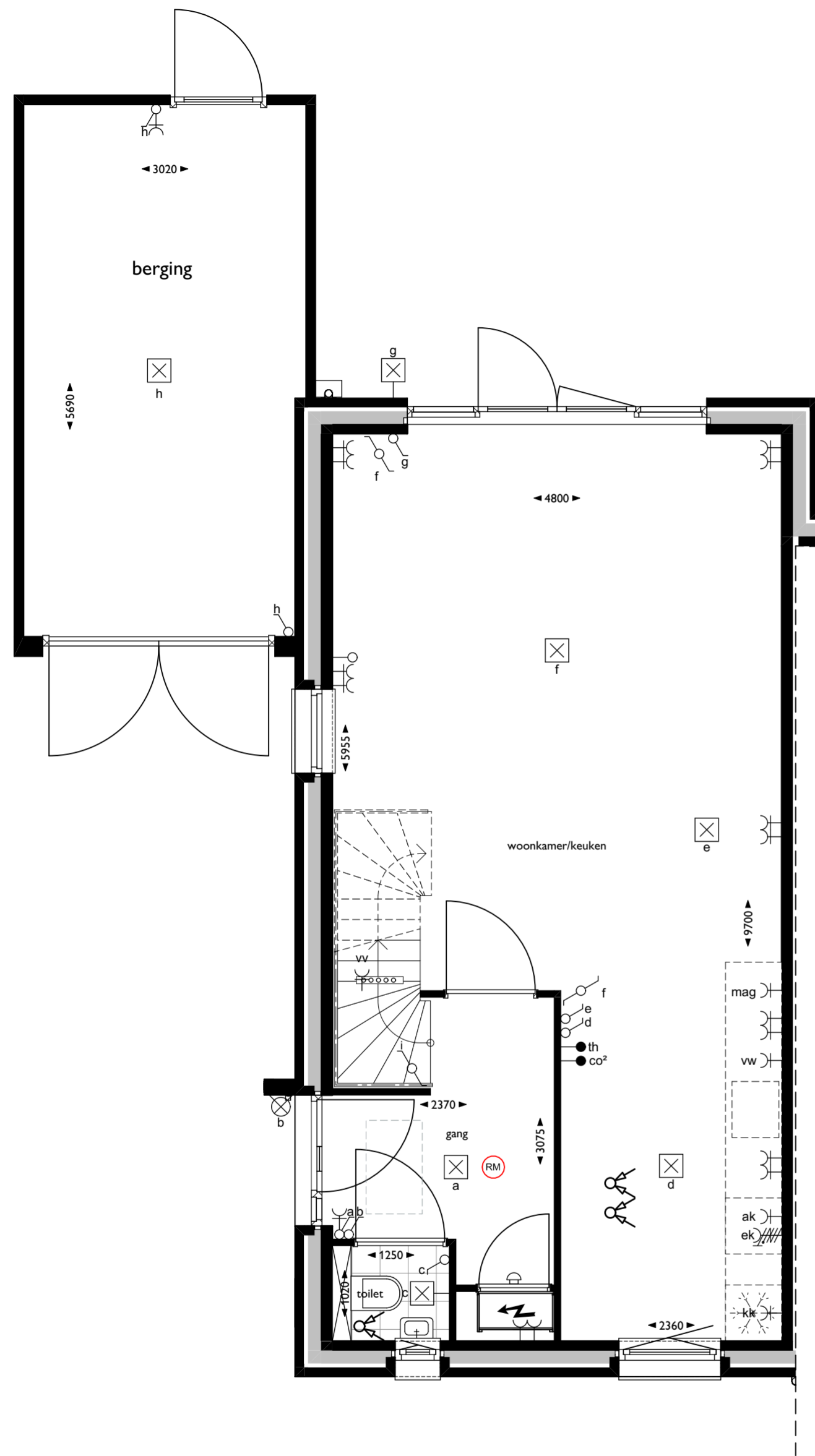
00 begane grond
